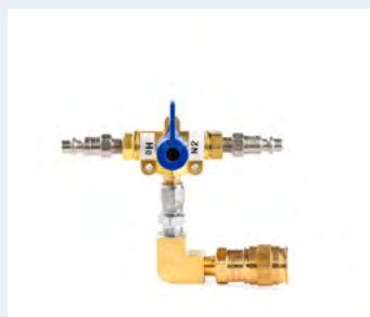
Helium/Nitrogen Quick Switch
